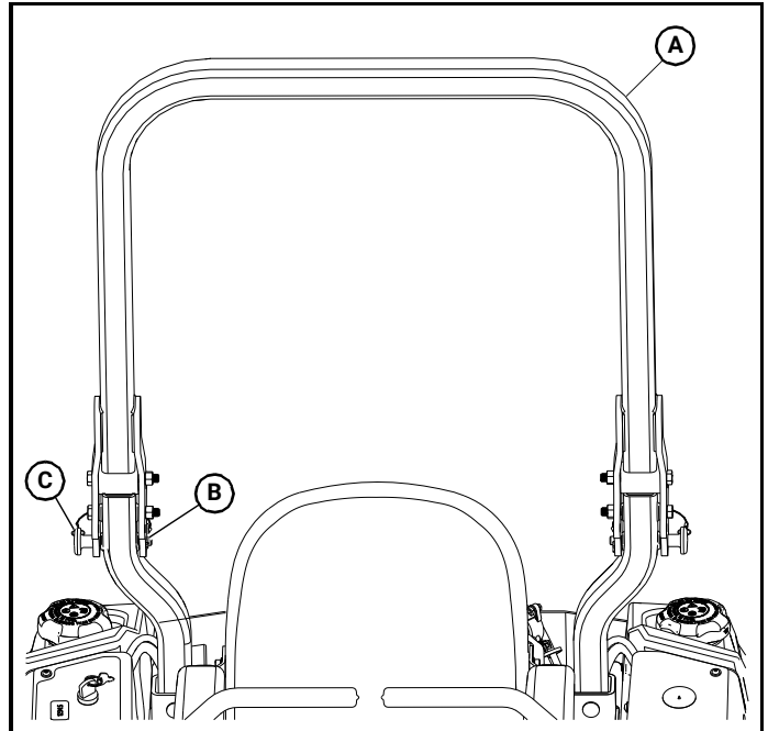
A. ROPS | B. Hair pin | C. Pin
